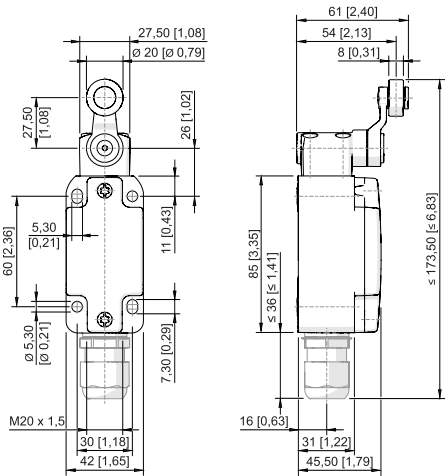
Swivelling lever 8070/2-3-D-U60
