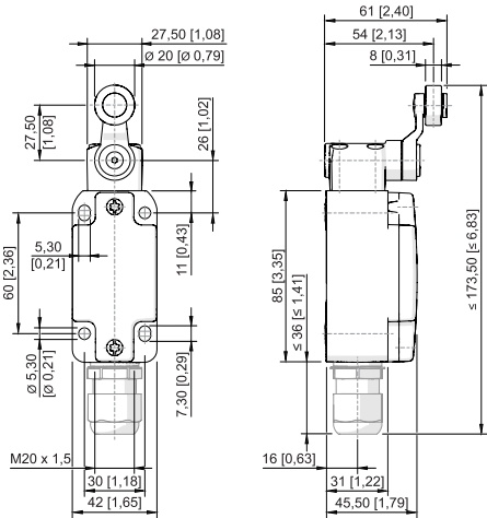
Swivelling lever 8070/2-1-D-U60
