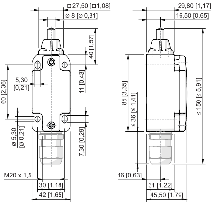
Domed plunger 8070/2-4-W-U60
