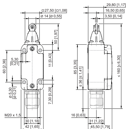
Roller plunger 8070/2-3-R-U60
