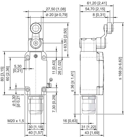
Swivelling lever 8074/2-D-40
