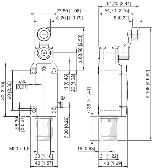
Swivelling lever 8074/2-5-D-40
