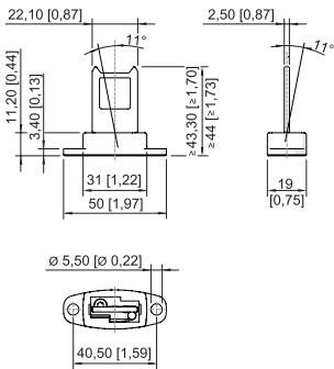
Movable actuator for safety switch
