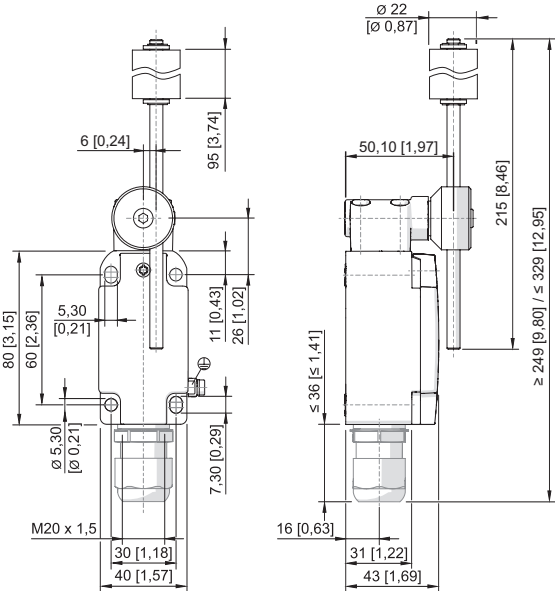
Misalignment switch 8074/2-1-SR-40
