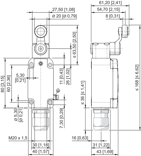
Swivelling lever 8074/2-1-D-40
