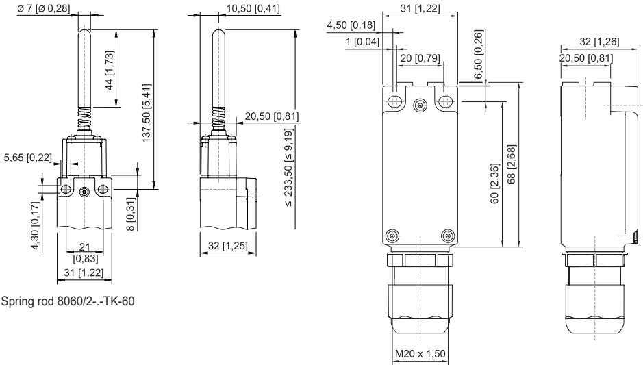
Snap-action contact, 1 NC + 1 NO 8060/-2; 807./2-2
