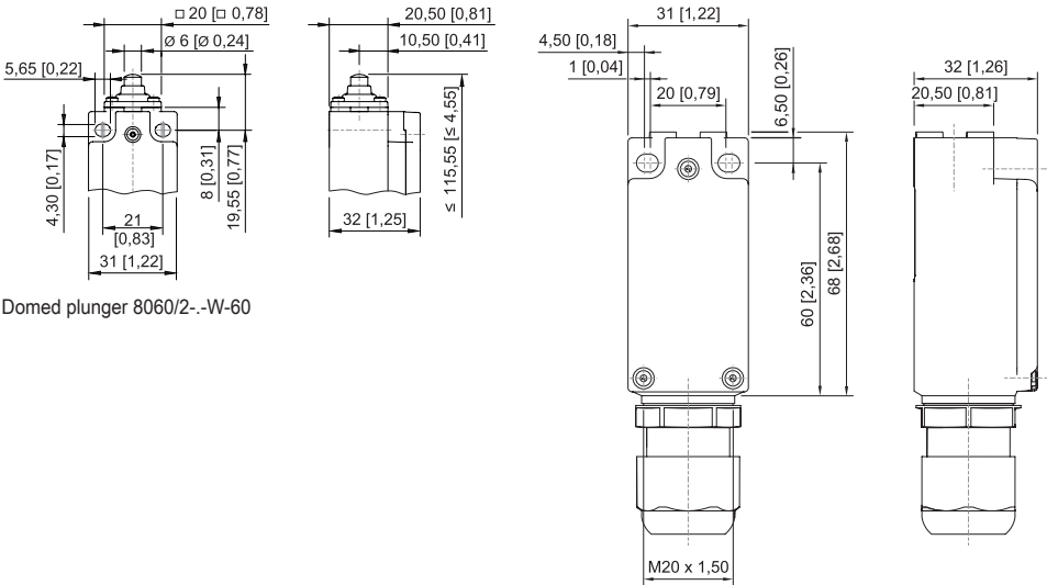
Slow-action contact, 1 NC + 1 NO 8060/-1; 807./2-1
