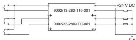
Application: Combination of potential-free contacts
