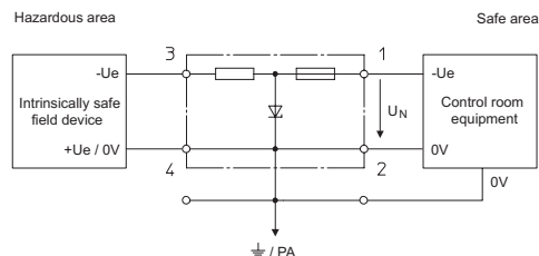
Single-Channel Safety Barriers for Negative Polarity
