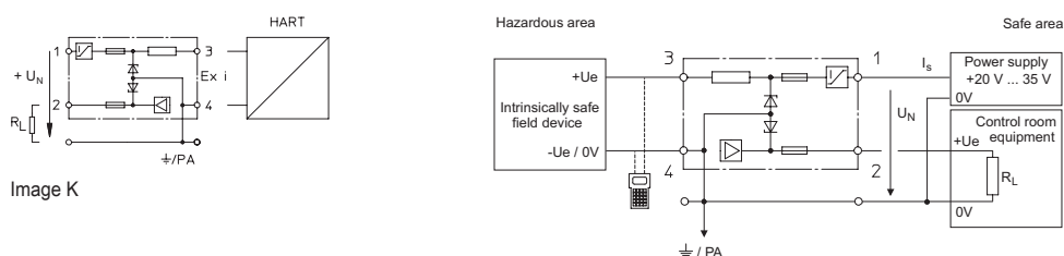
Single-Channel Safety Barriers for Transmitters
