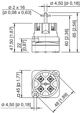
8008/2-0 1- or 2-pole control switch
