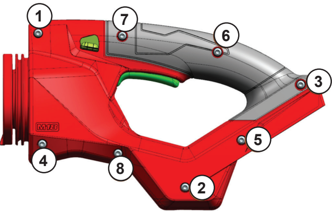
STEP 5 - Back Handle Cover
