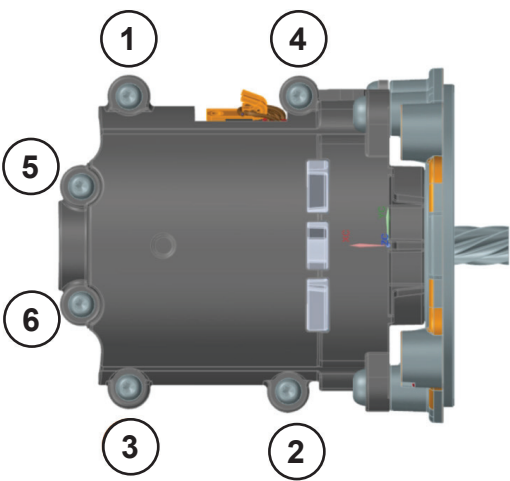
STEP 10 - Motor Housing
