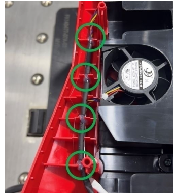
WIRE ROUTING AND GLUING OF FANS
