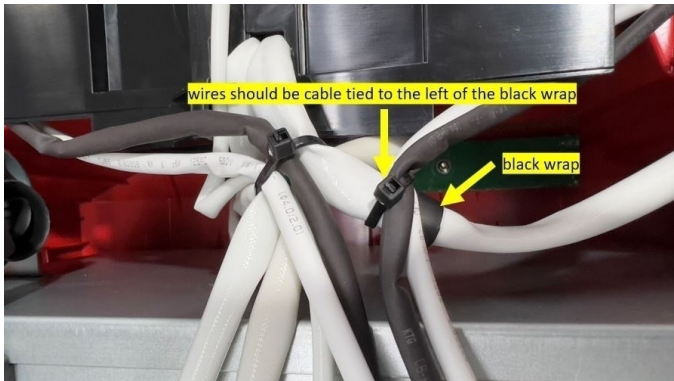
USE TWO CABLE TIES TO FASTEN THE WIRES AS BELOW
