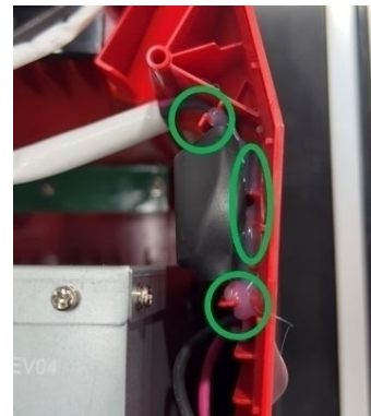
WIRE ROUTING AND GLUING OF THE FERRITE BEAD
