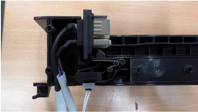
WIRE ROUTING OF THE WIRES BETWEEN THE INTERFACES
