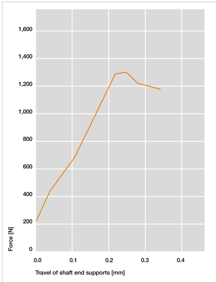
Axial compressive strength of the split fixing collar up to 1,300N
