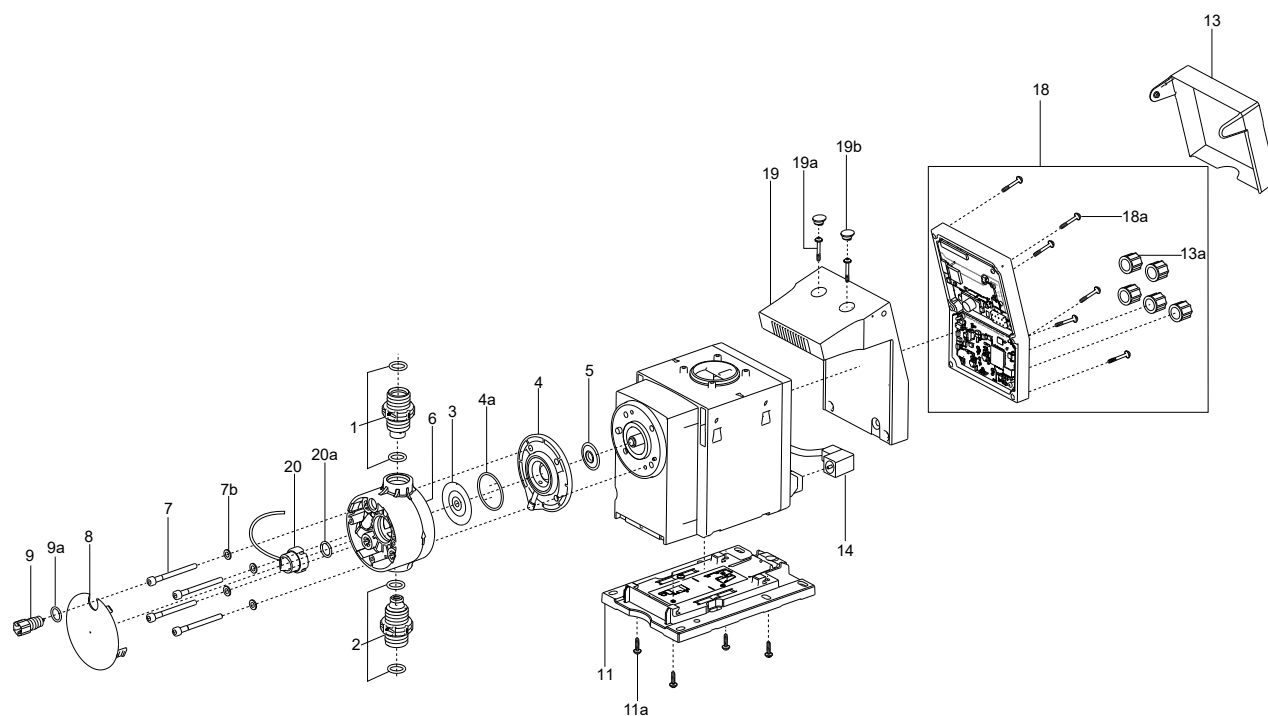
Exploded view for DDA-C, up to 17 l/h
