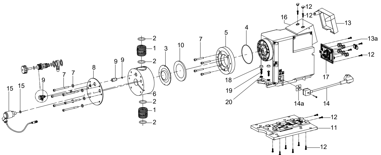
Exploded view for DDA, DDE, 120 - 200 l/h
