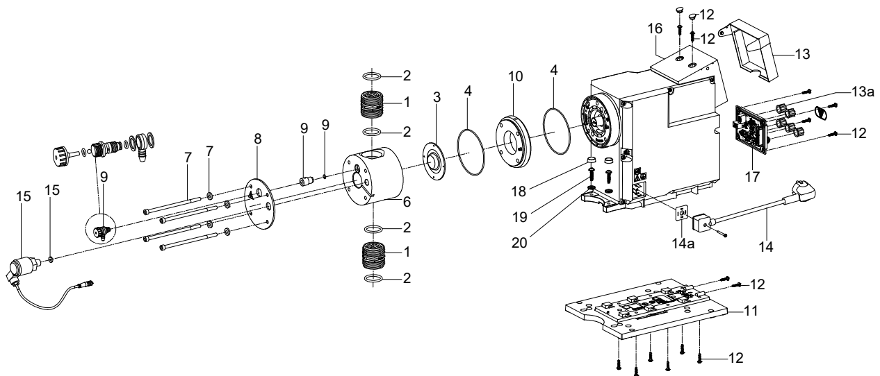
Exploded view for DDA, DDE, 60 l/h
