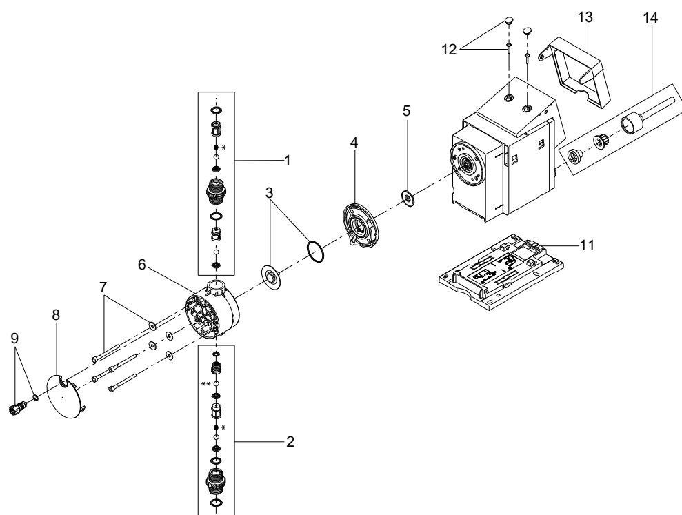
Exploded view for DDA, DDC, DDE, up to 17 l/h
