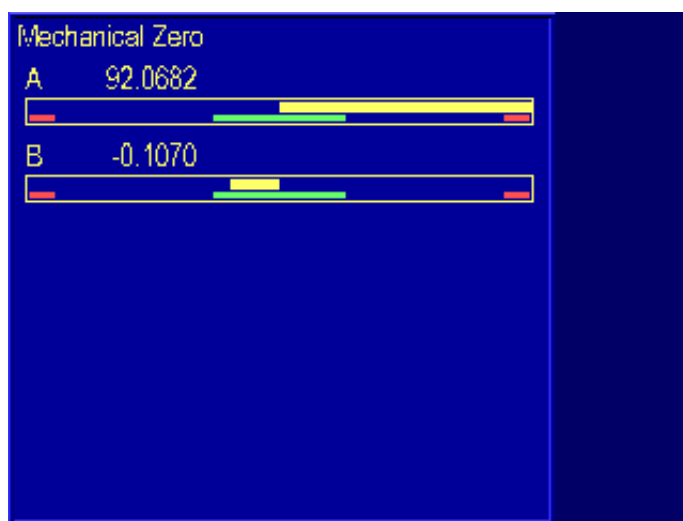
Figure 6-6. Mechanical Zeroing Screen
