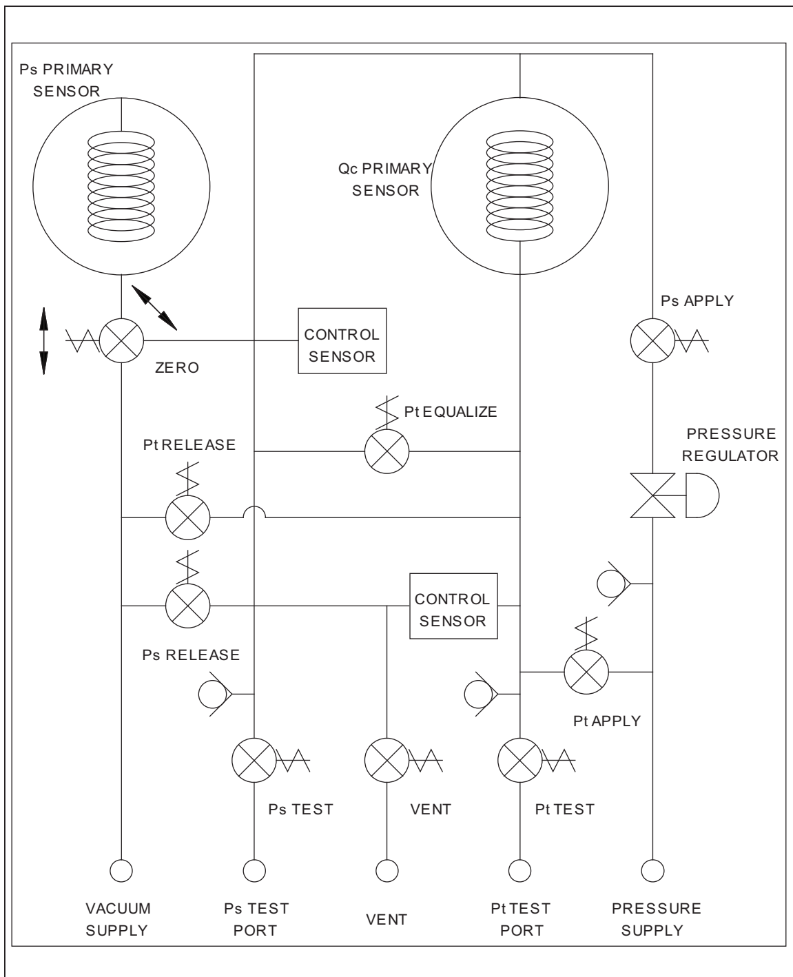
Figure 2-3. RUSKA 7750i ADTS - Pneumatics Schematic Diagram
