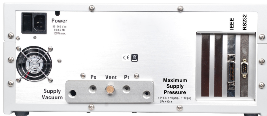
Figure 3-1. RUSKA 7750i Back Panel
