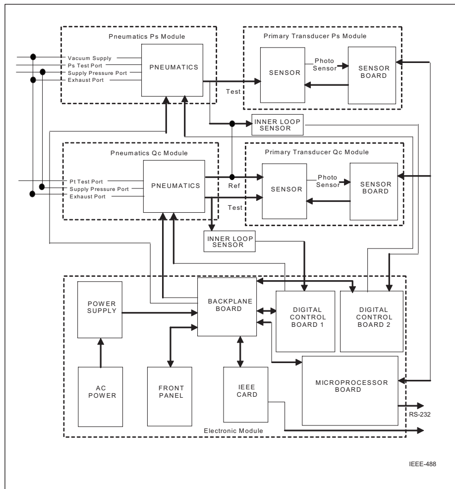
Figure 2-1. ADTS Block Diagram
