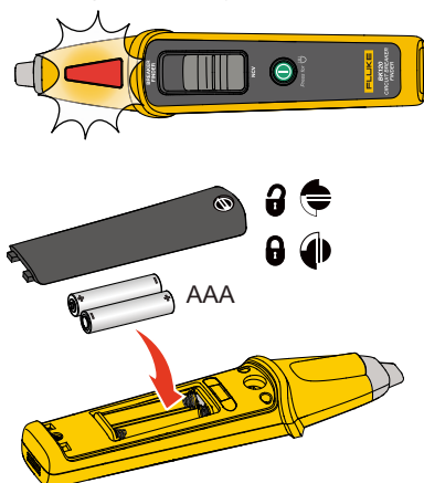
Figure 14. Battery Replacement
