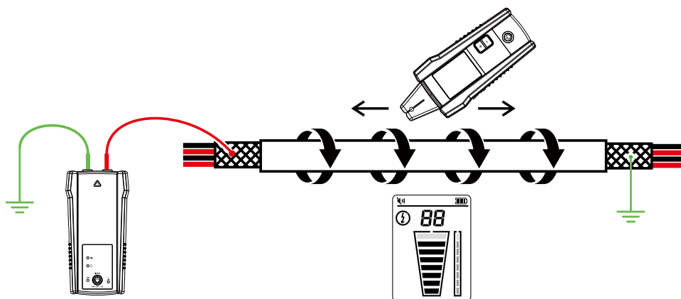
Figure 4.6a: Tracing a shielded wire grounded at the far-end
