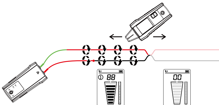
Figure 4.3: Tracing a cable to find shorts
