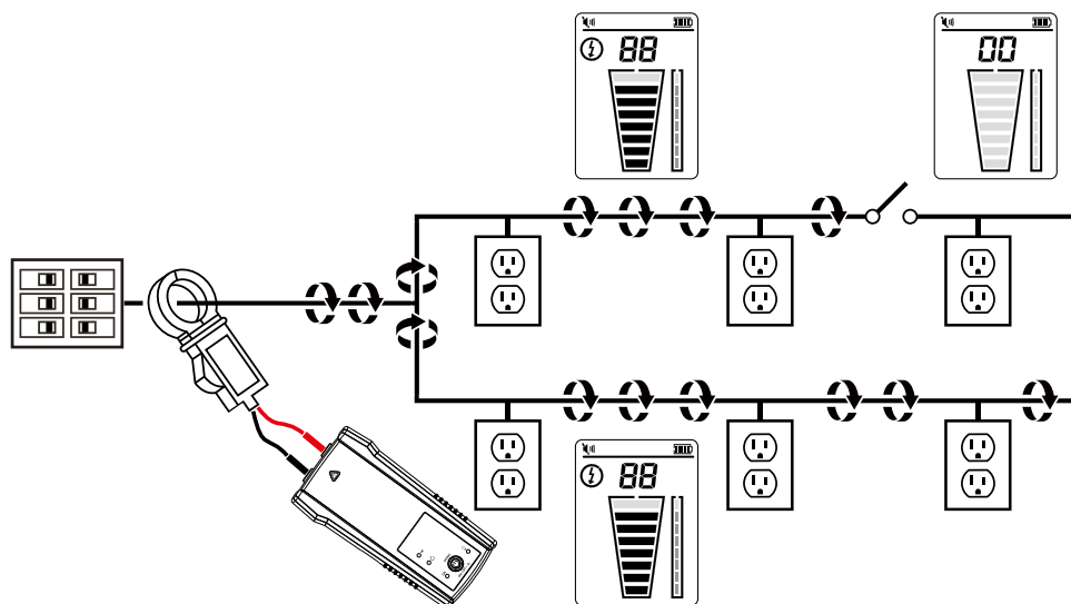
Figure 4.13: Using the Signal Clamp to map loads to specific breakers
