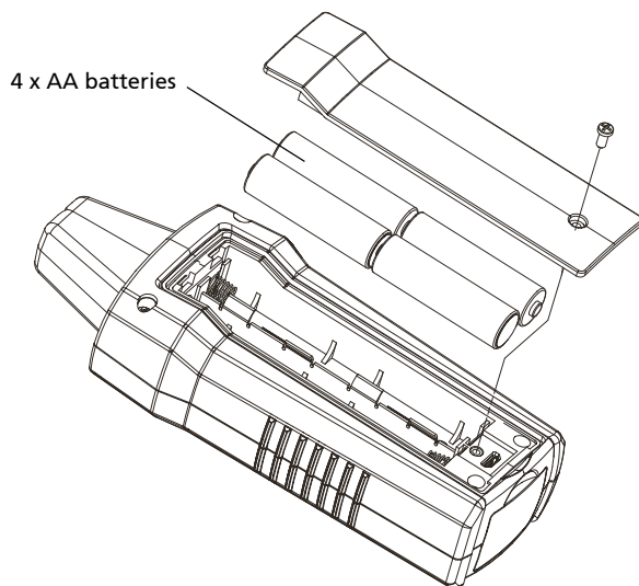
Figure 5.1b: Changing the Receiver batteries
