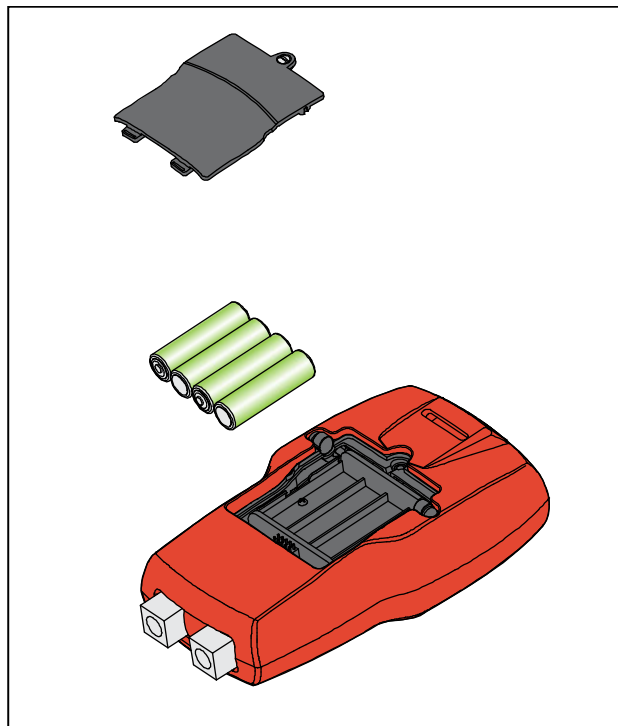
Figure 8. Battery Replacement
