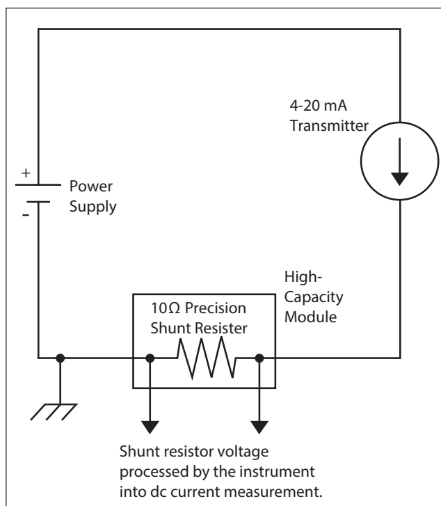
Figure 1. Current Shunt Resistor in a Two-Wire Transmitter Measurement Loop
