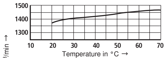
Temperature dependency at \Delta p = 20 bar
