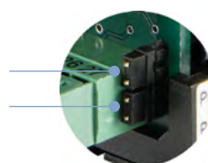
Jumper 2 (NPN/PNP)
