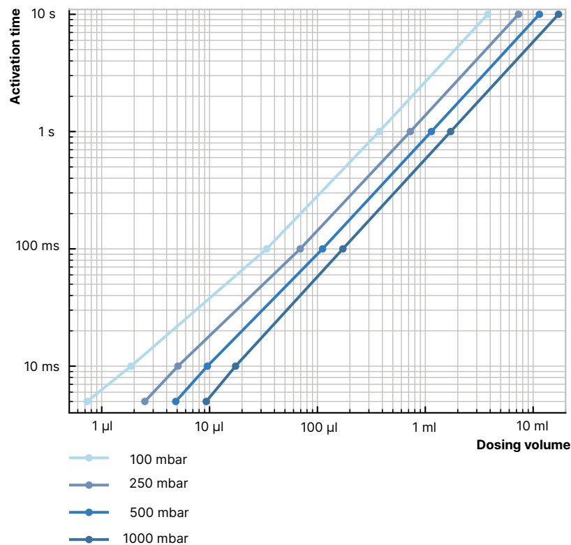
Dosing needle with 0.51 mm diameter, Type 6650, DN 0.8
