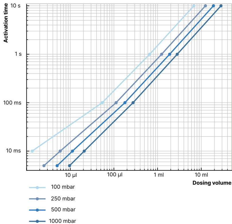
Dosing needle with 0.95 mm diameter, Type 6650, DN 0.8
