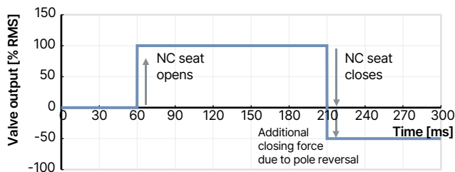
Valve voltage curve
