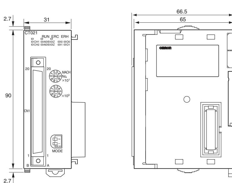
Dimensions with Connector
