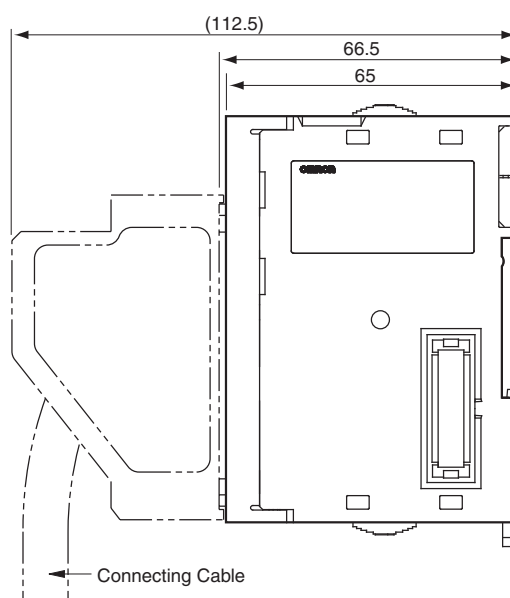
Dimensions with Connector
