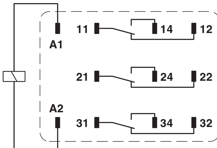
Koblingsplan
