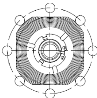
DN 65 – 100
