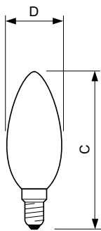
Candle B35 2-25W 250lm4000K E14 ND Clear
