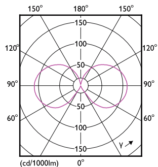
Candle B35 2-25W 250lm4000K E14 ND Clear
