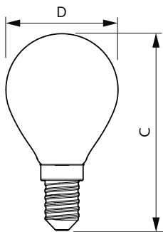
Candle P45 60W 806lm 4000K E14 NDFrosted
