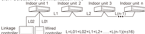
Fig.5.3 Length of communication wire
