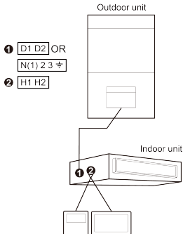
Fig. 5.5 one linkage controller and one wired controller control one indoor unit
