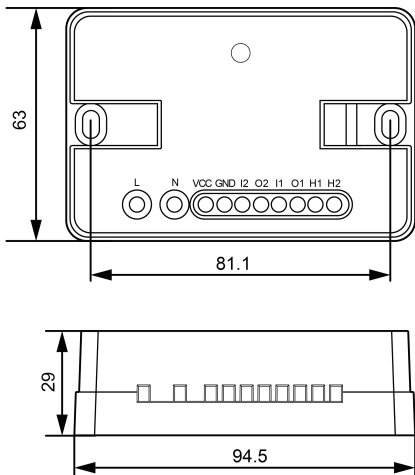
Fig.5.1 Dimensions of Product
