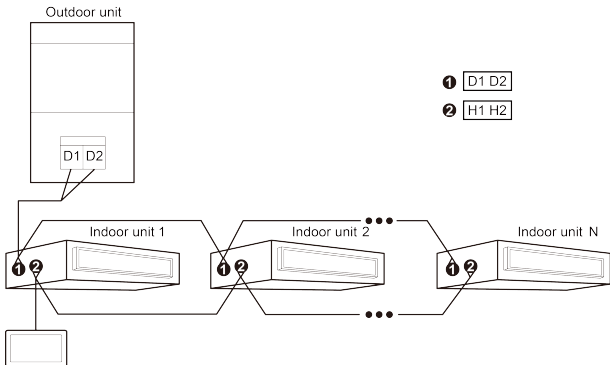
Fig. 5.6 one linkage controller controls multi VRF indoor units simultaneously
