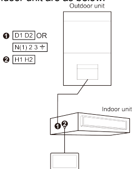
Fig. 5.4 one linkage controller controls one indoor unit
