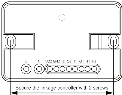
Fig.5.2 Installation Means
