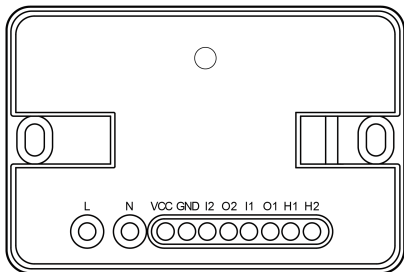
Fig.3.1 Exterior Sketch of Linkage Controller
