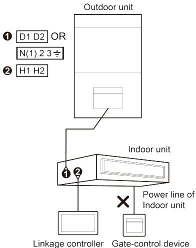
Fig.5.11 Wrong Connection 2 of Units and Gate Control
