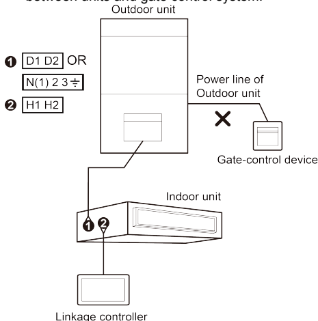
Fig.5.10 Wrong Connection 1 of Units and Gate Control
