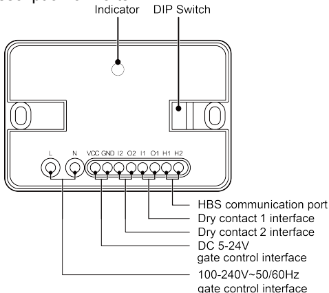
Fig.4.1 Diagram of Ports
