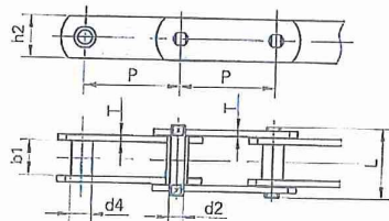
4.with F flanged rollers type
