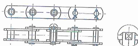
5.Welded pins with plates
