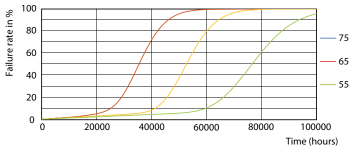
Life Expectancy Diagram - MAS LEDtube 1200mm UO 14.7W 840 T8
