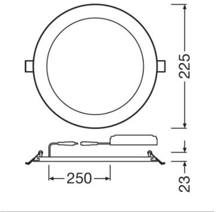
DL SLIM ALU DN 205 22 W 3000 K WT, DL SLIM ALU DN 205 22 W 4000 K WT
