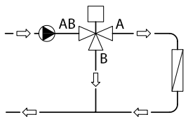
Fig. 4: Diverting valve used in diverting application
