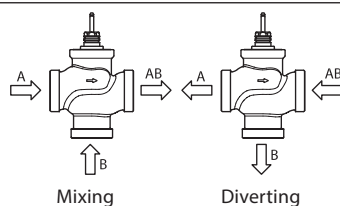
Fig. 1: Mixing or diverting connection
