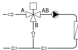
Fig. 2: Mixing valve used in mixing application
