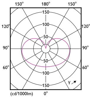
Light Distribution Diagram - MAS VLE LEDLusterD3.4-40W E27 P45 927FRG
