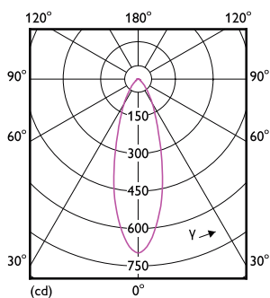
LEDspots Corepro SLR 4W PAR16 GU10 840 36D-LDD
