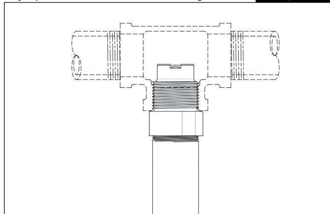
Dry Sprinkler Protrusion into Fitting
