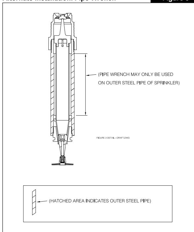
Alternate Installation: Pipe Wrench
