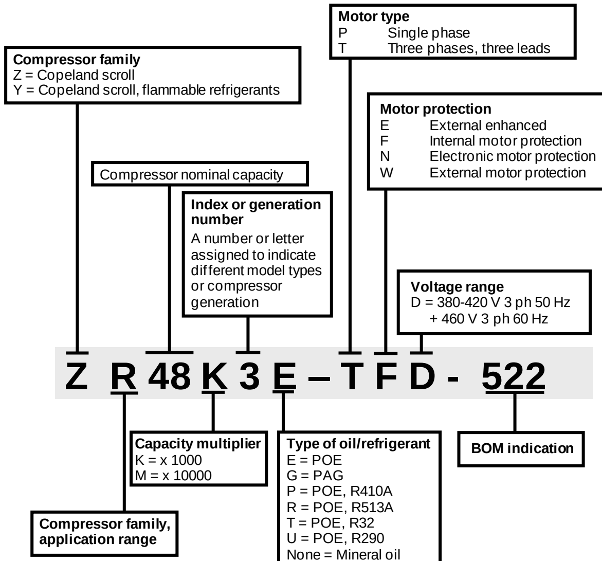
Figure 1: Example of nomenclature for a standard scroll compressor, ZR range
