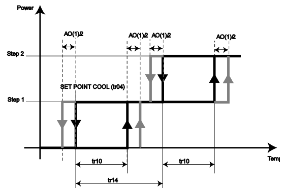
Setpoint and hysteresis modification after calculation of AO1
