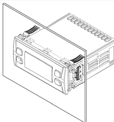
Panel-mounted SB series • SKP 10
