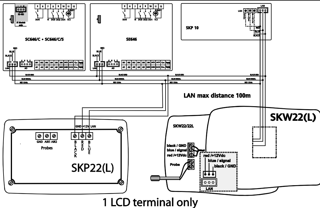
connection SC600 - SE600 - SKP10 – LCD terminal
